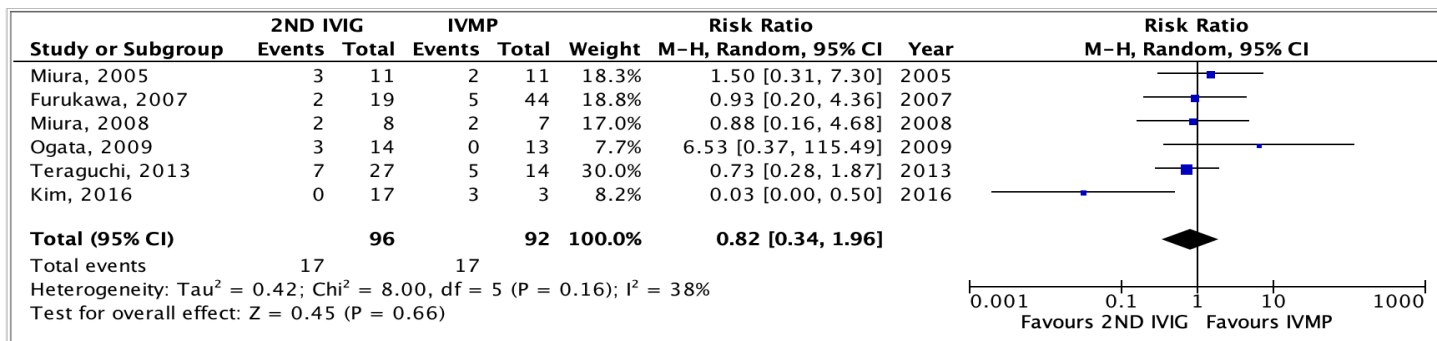
Figure 3. Forest plots of a traditional pair-wise meta-analysis of CALs post-treatment in patients with refractory KD
