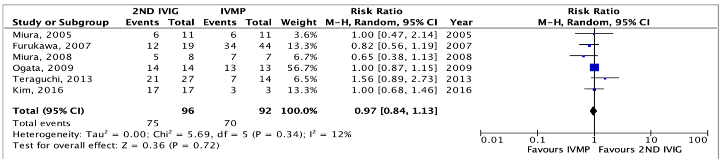
Figure 4. Forest plots of a traditional pair-wise meta-analysis of fever resolution post-treatment in patients with refractory KD
